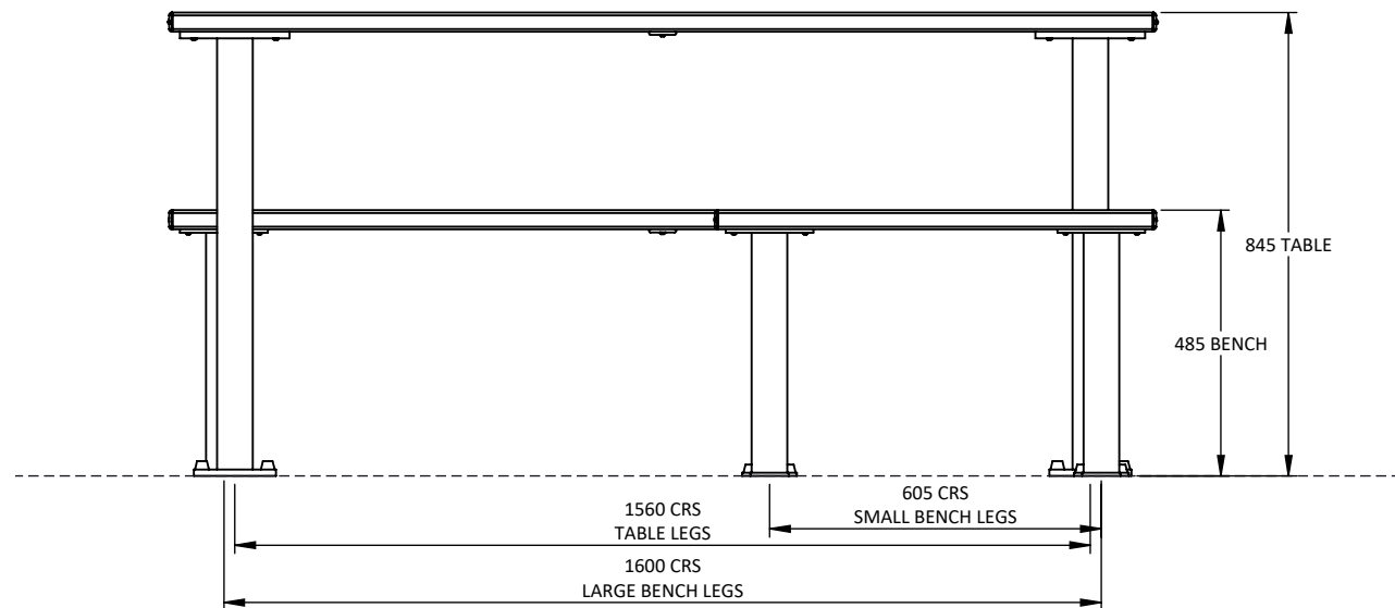
FRONT VIEW
