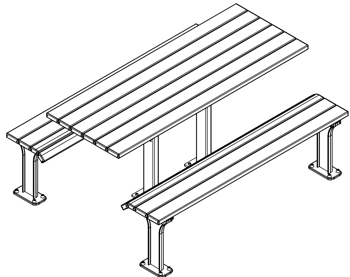
DIMETRIC VIEW
