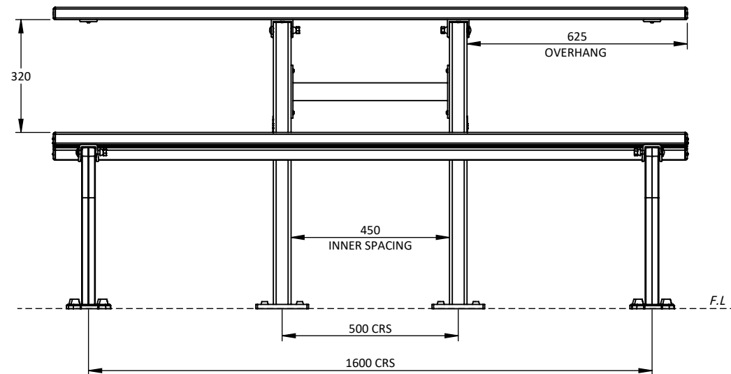
FRONT VIEW
