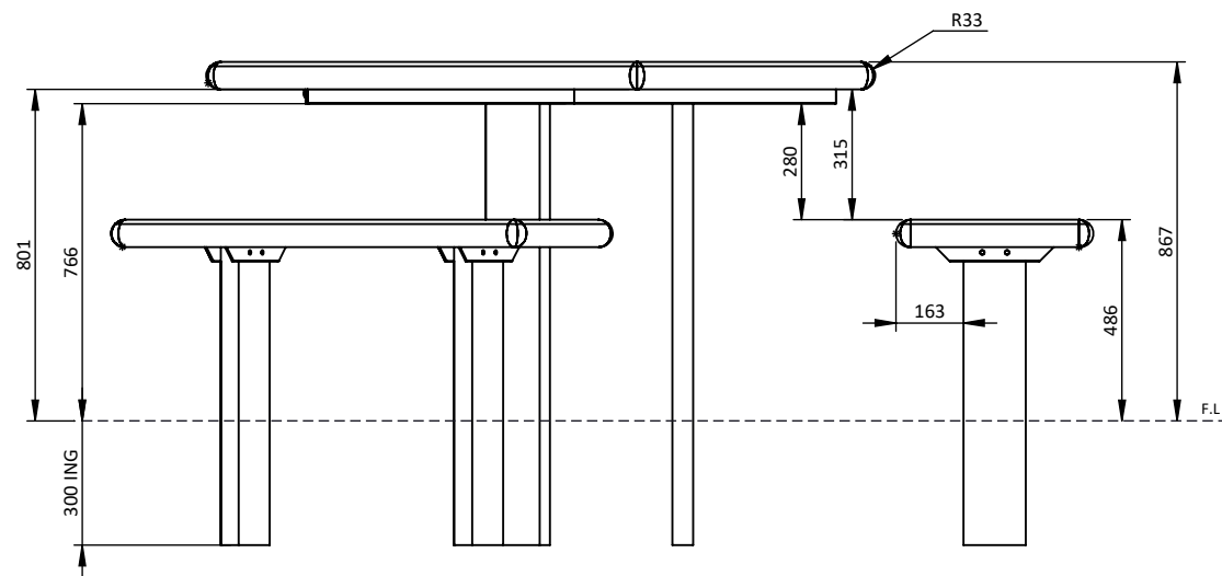
SIDE VIEW
