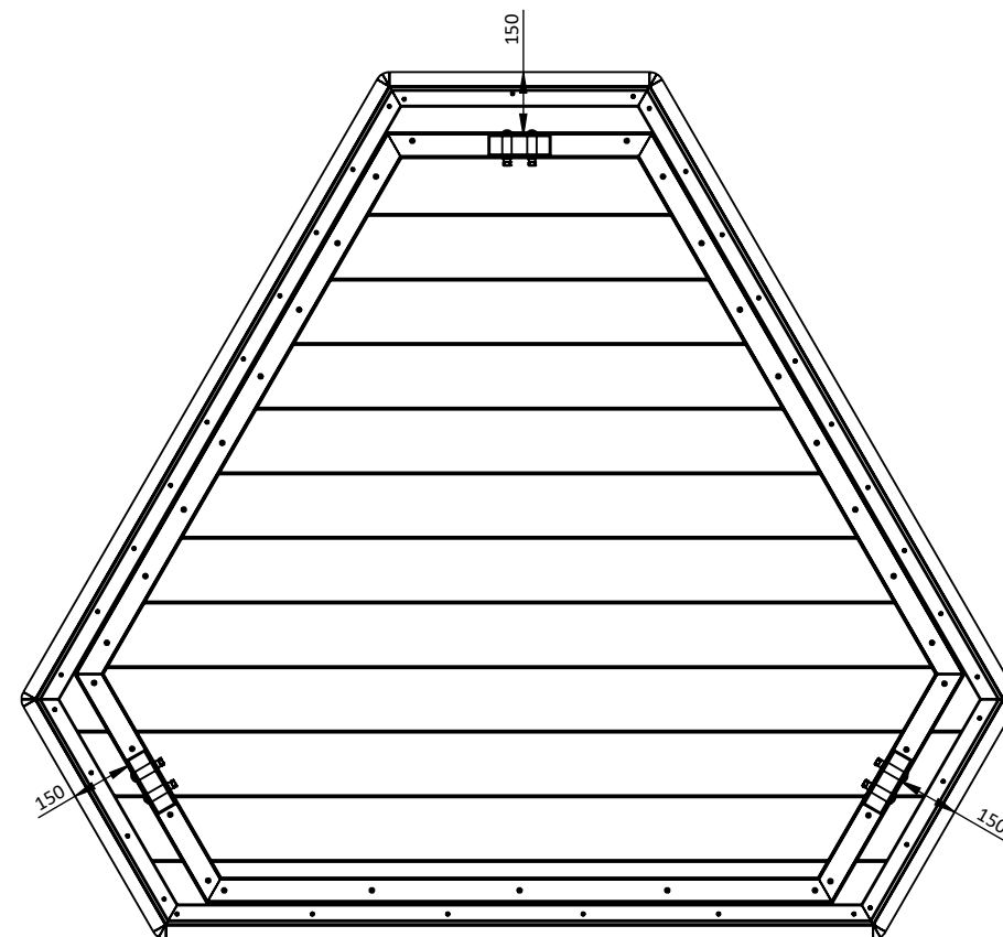
BOTTOM VIEW
