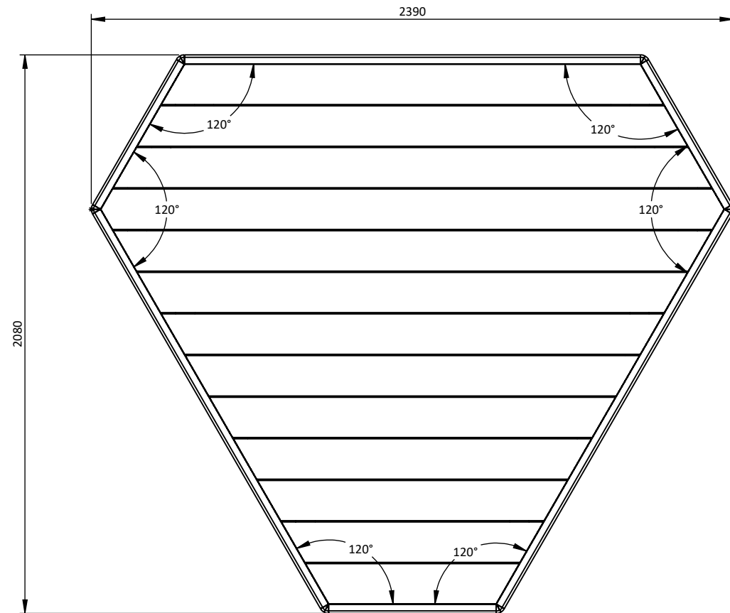
TOP VIEW
