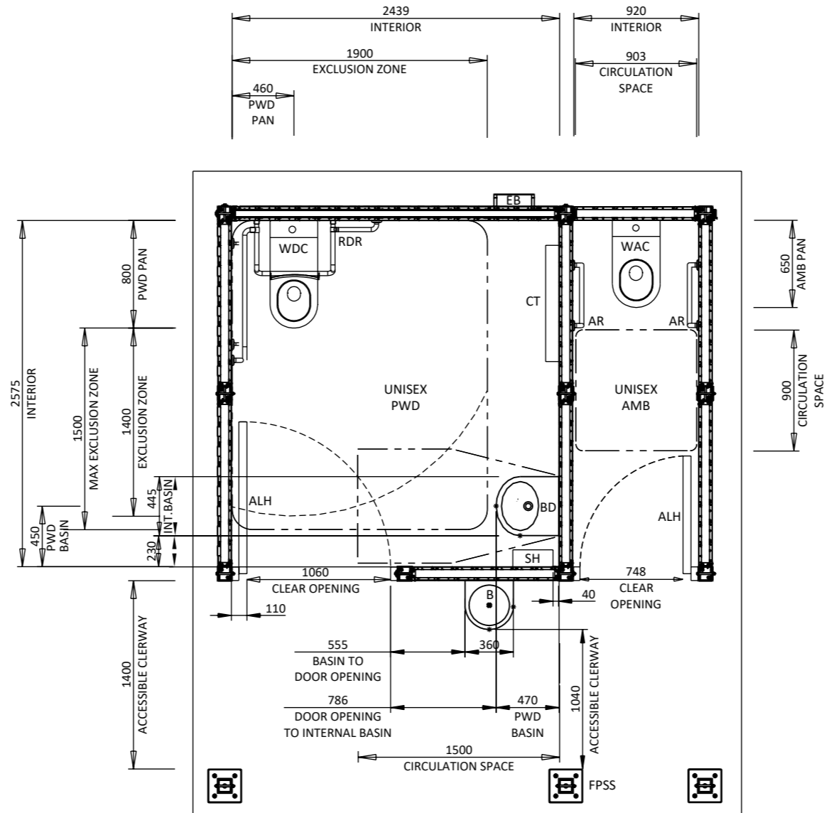
FLOOR PLAN 1:40
