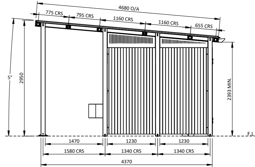
SIDE VIEW 1:55
