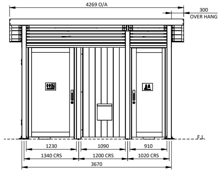
FRONT VIEW 1:55
