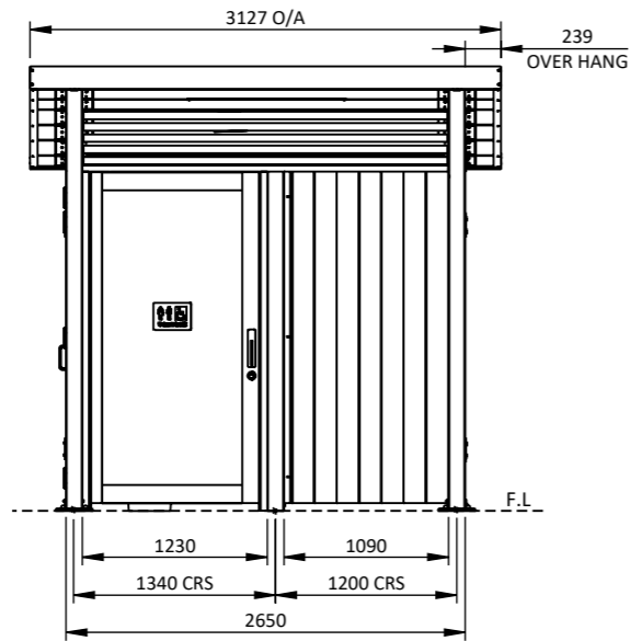
FRONT VIEW 1:55
