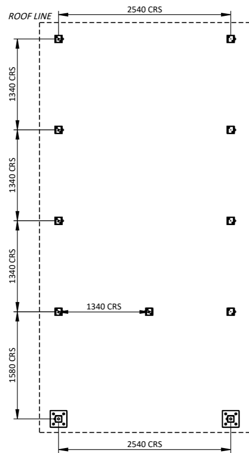
FOUNDATION PLAN 1:55
