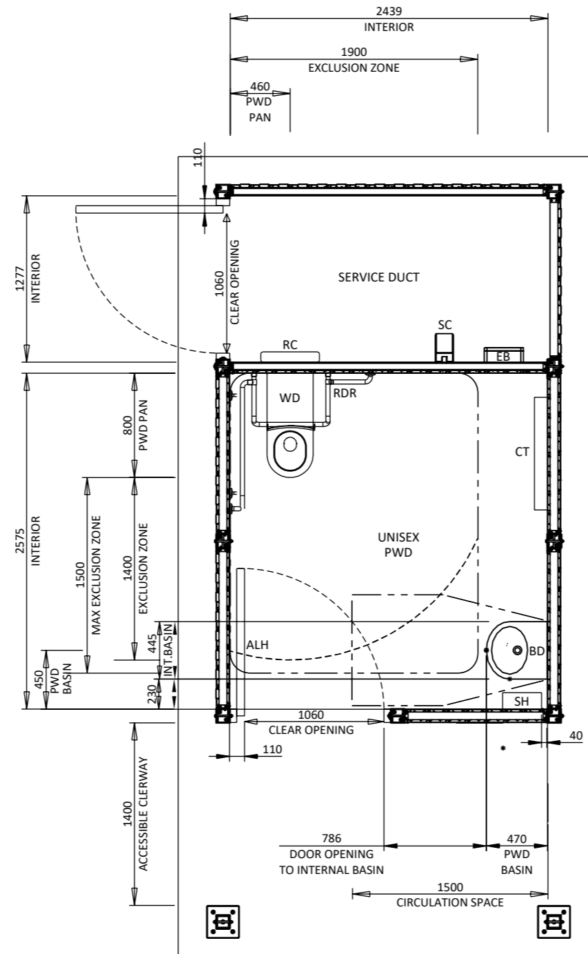
FLOOR PLAN 1:40
