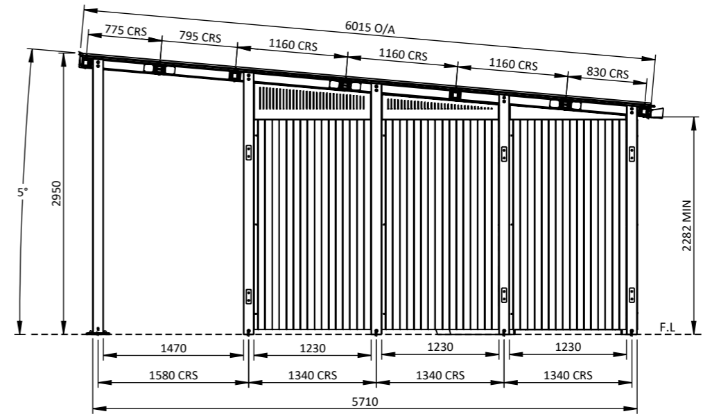
SIDE VIEW 1:55
