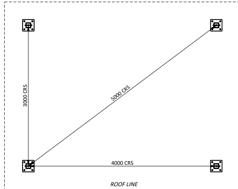
FOUNDATION PLAN 1:50
