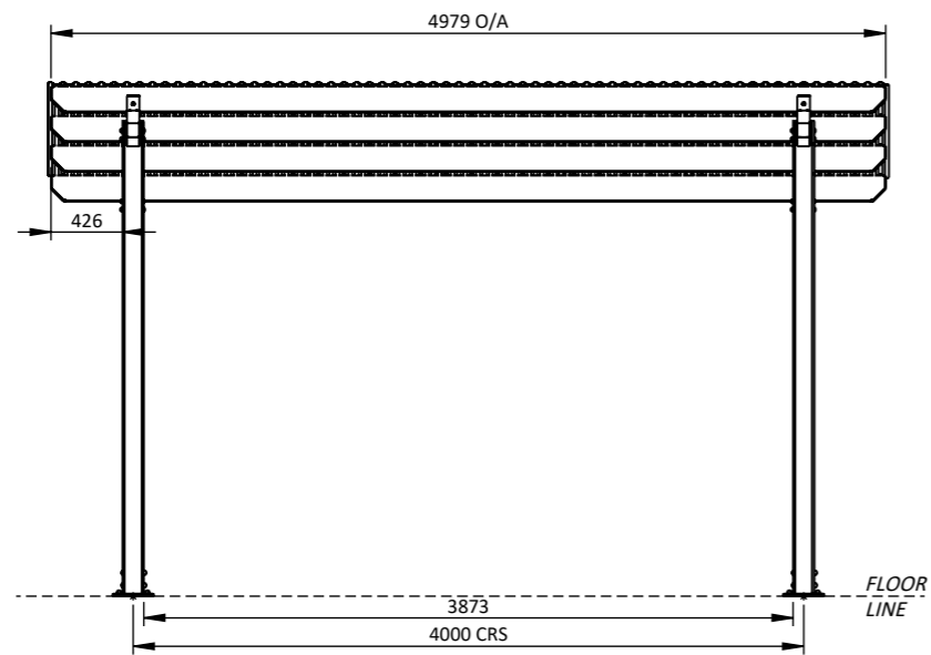
FRONT VIEW 1:50
