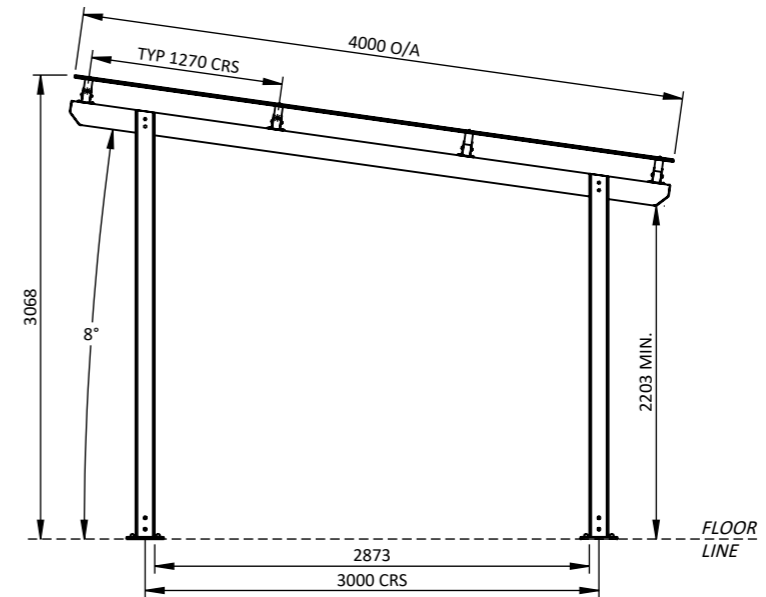
SIDE VIEW 1:50
