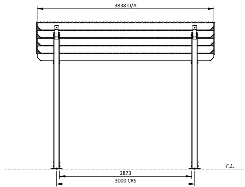
FRONT VIEW 1:50
