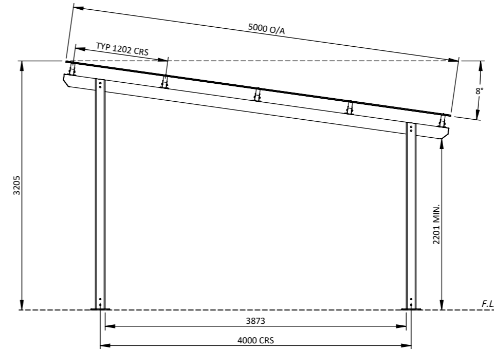
SIDE VIEW 1:50
