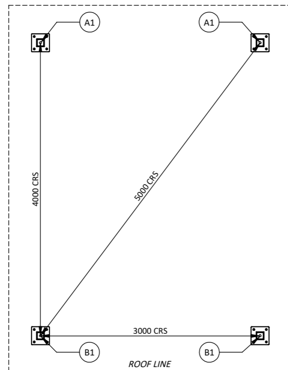
FOUNDATION PLAN 1:50
