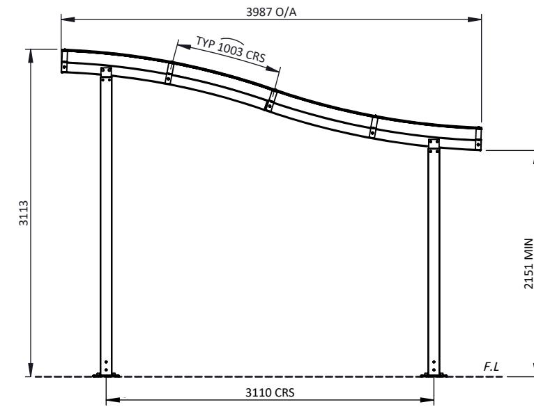
SIDE VIEW 1:50
