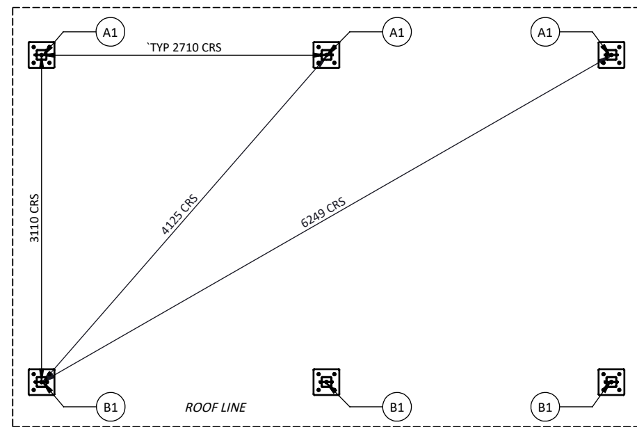
FOUNDATION PLAN 1:50
