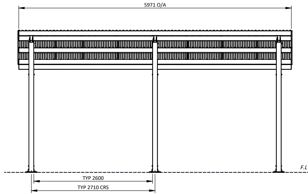
FRONT VIEW 1:50
