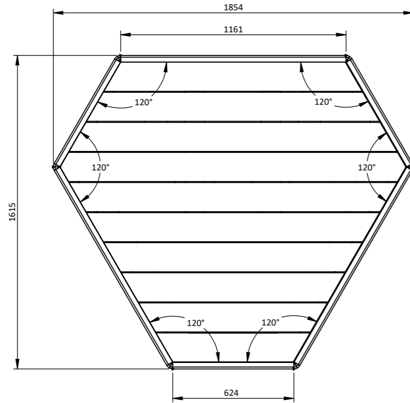
TOP VIEW 1:20
