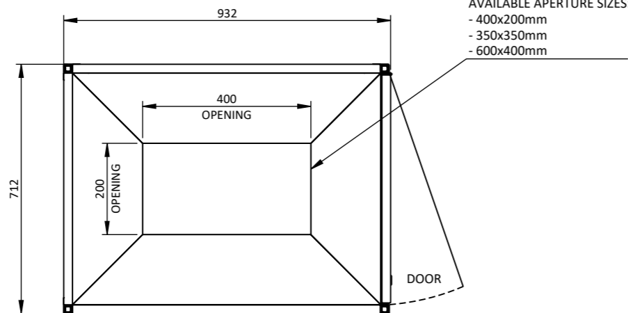
○ SIDE - TOP VIEW
