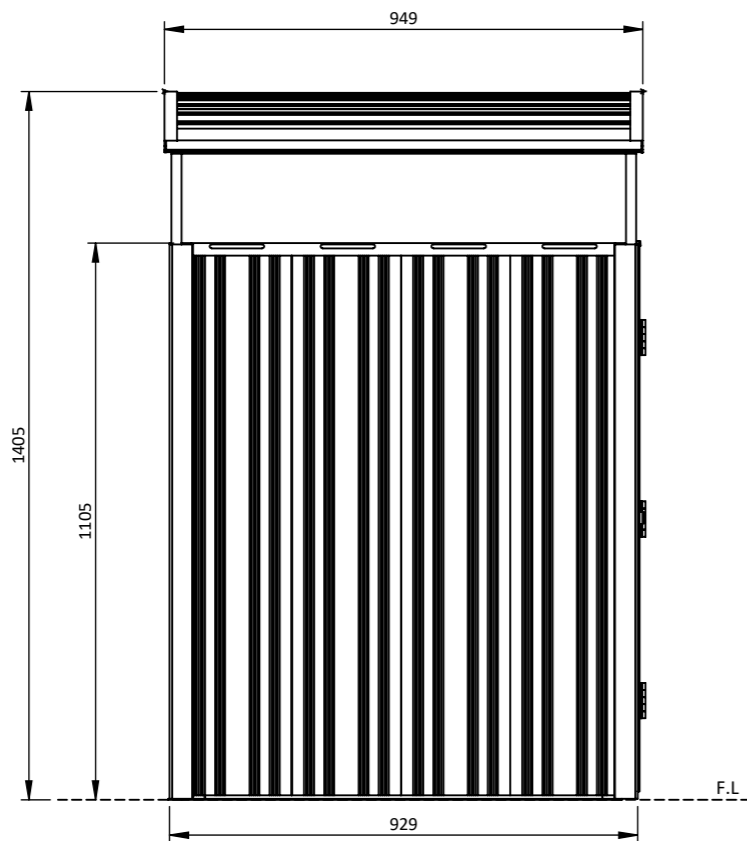
FRONT ELEVATION 1:15
