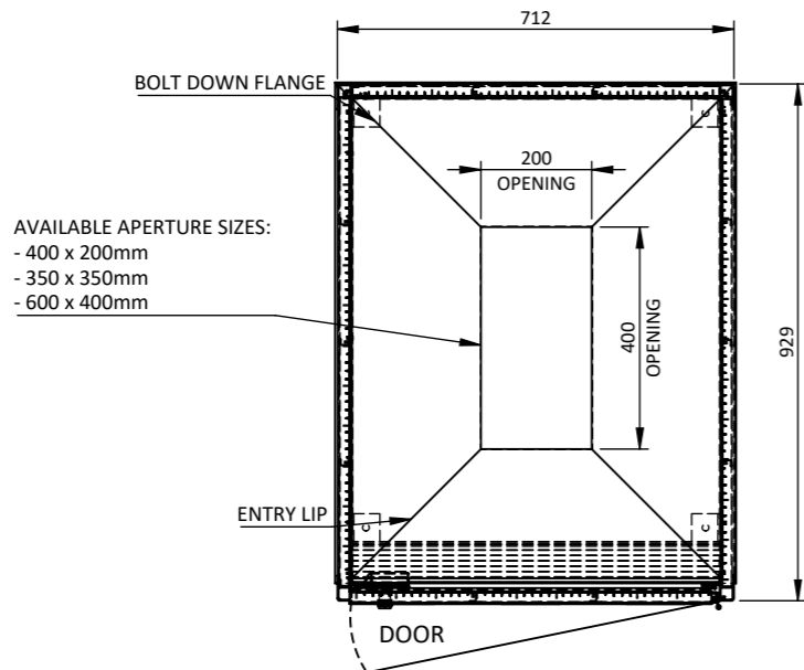
PLAN VIEW 1:15
