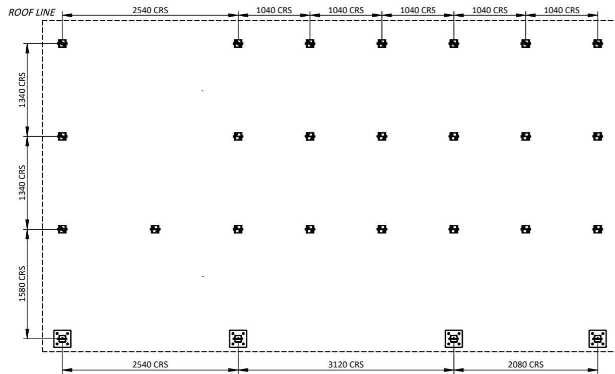
FOUNDATION VIEW 1:55
