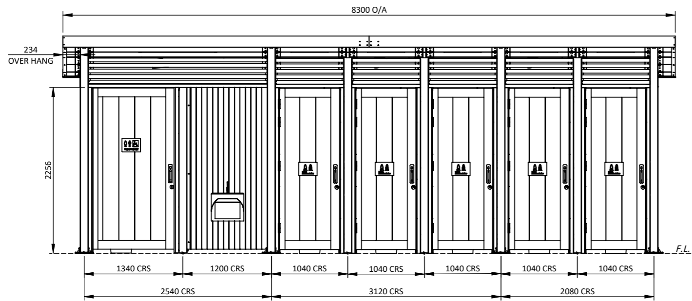
FRONT VIEW 1:55
