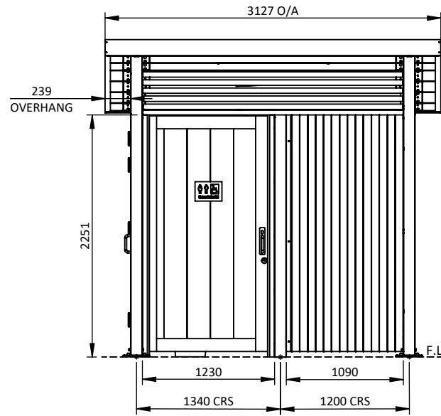
FRONT VIEW 1:50
