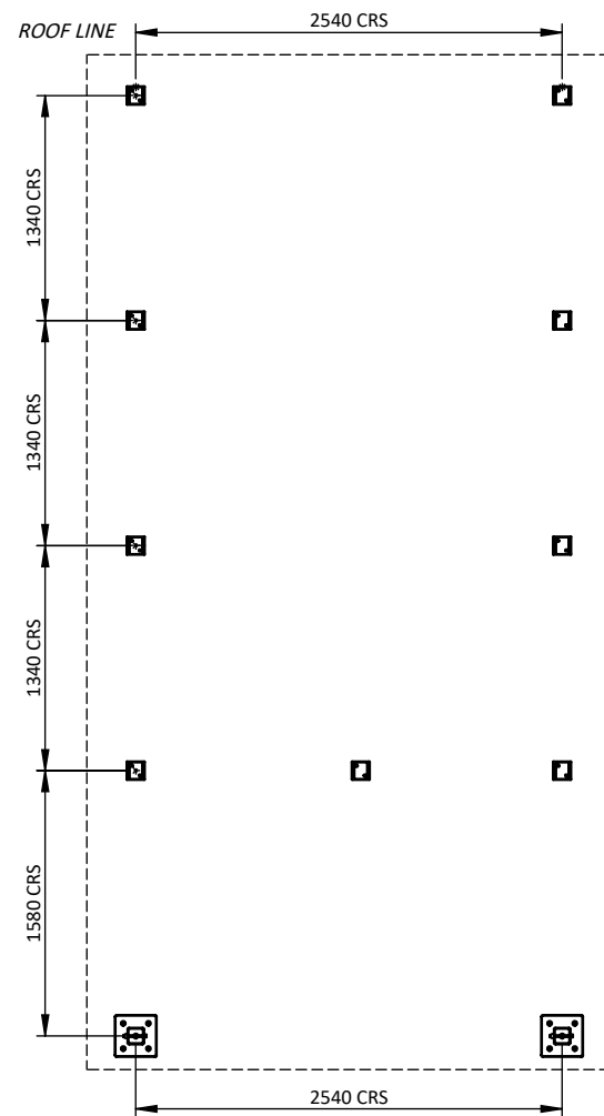
FOUNDATION PLAN 1:50
