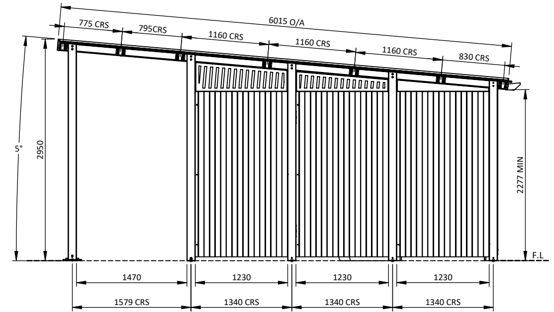
SIDE VIEW 1:50
