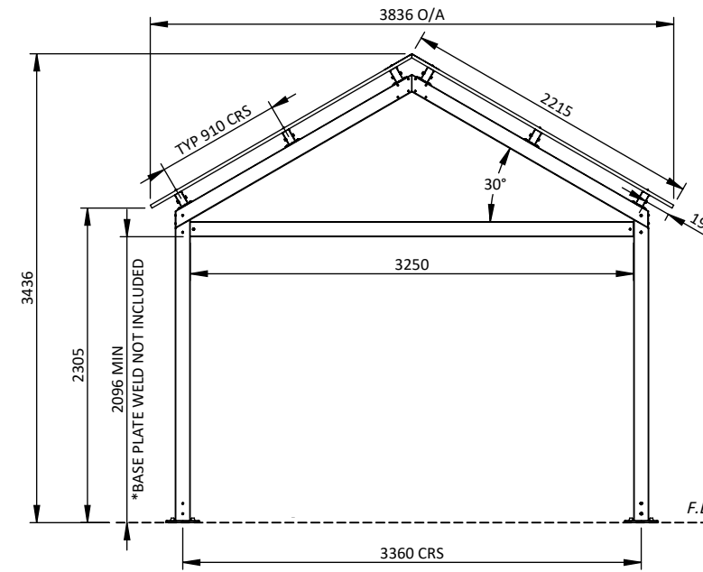
SIDE VIEW 1:50
