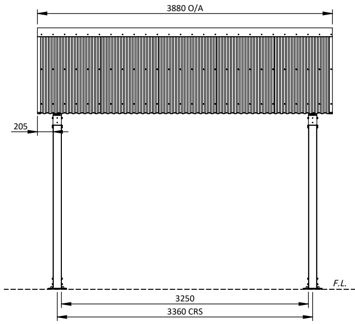
FRONT VIEW 1:50
